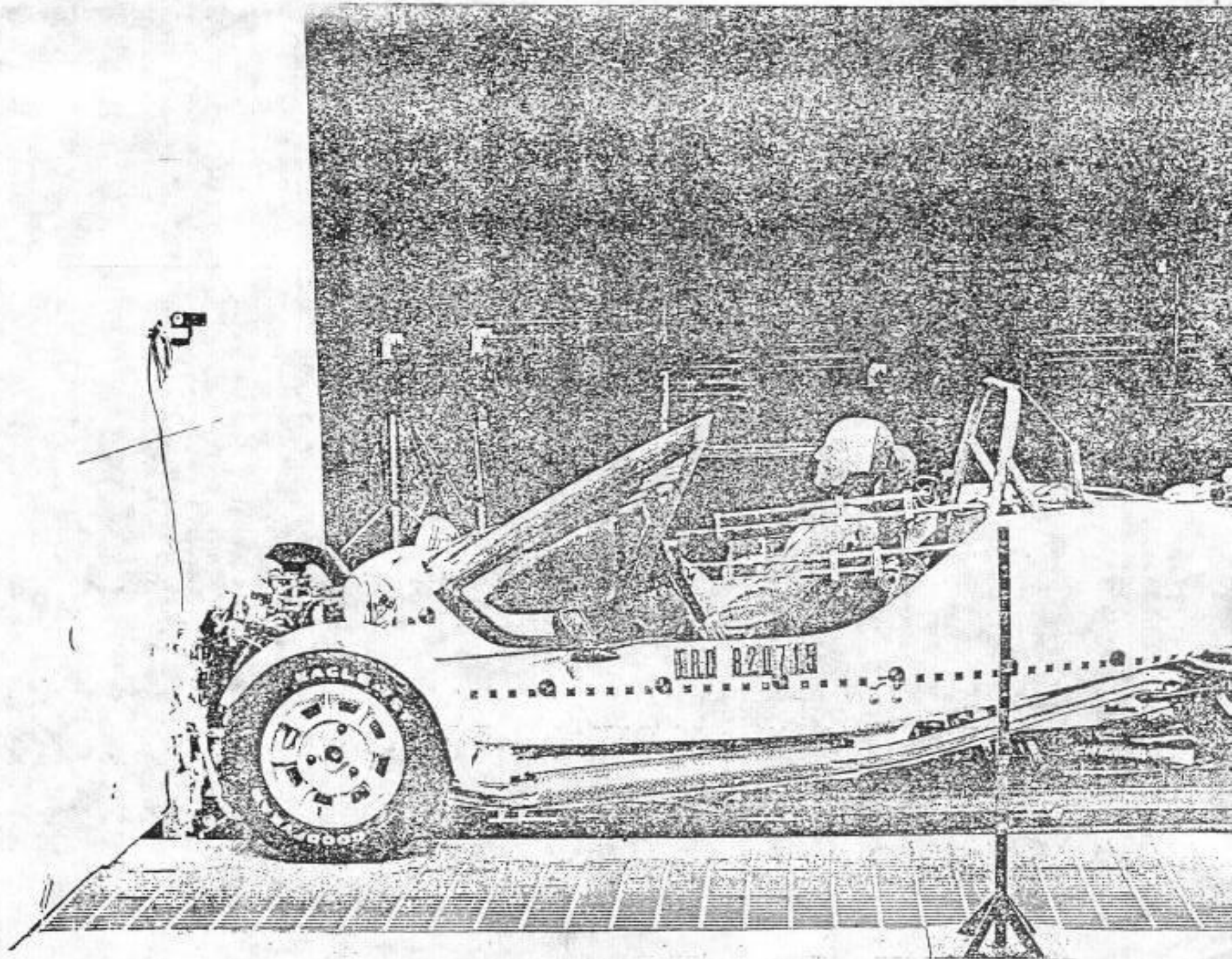
Figure A-6. POST-TEST LEFT SIDE VIEW
